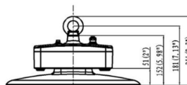
Hook Mounting
